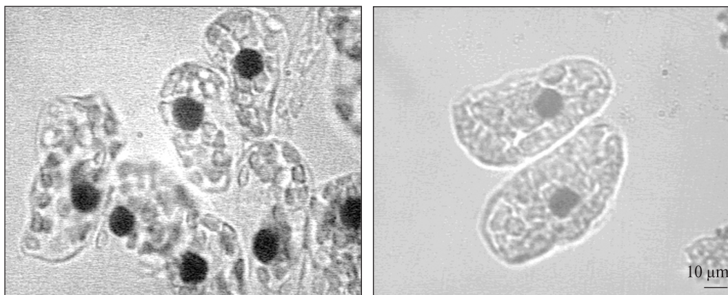
Fig. 2. The parenchyma leaf cells of D. antarctica stained for nuclear area and DNA content measure according to Feulgen
